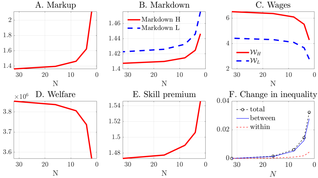
Figure 1: Comparative Statics
